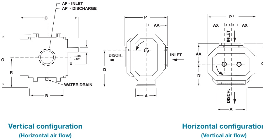
Outline drawing of Roots VJ WHISPAIR water sealed exhauster.
